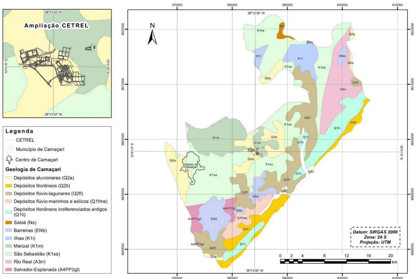
Figure 4. Geological map of the municipality of Camaçari and the CETREL region.
