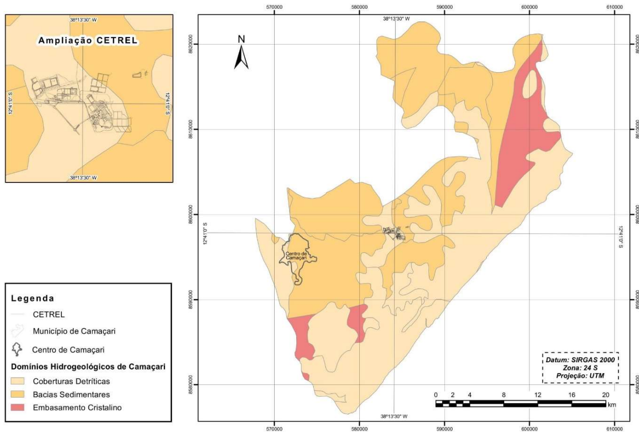
Figure 5. Map of hydrogeological domains of the municipality of Camacari and the CETREL region.
